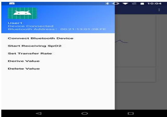
Fig 3. App interface 1
