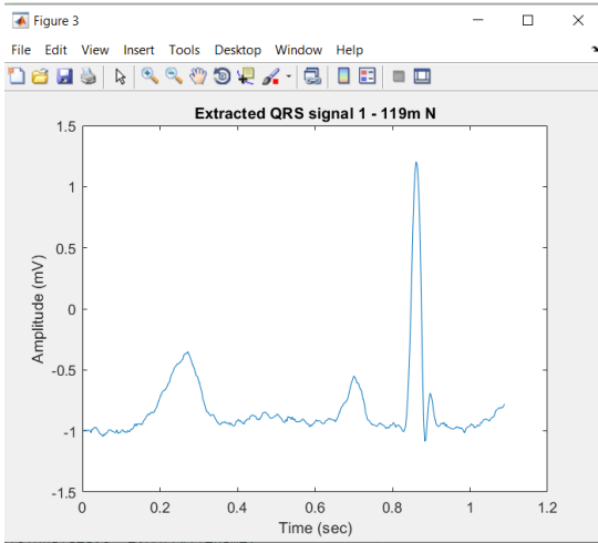
Fig 5. Feature extraction
