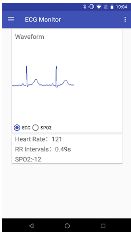
Fig 4. App interface 2
