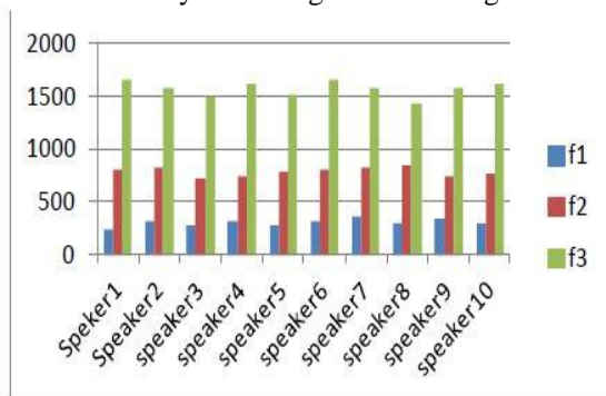
Fig.8. Formants f1,f2 and f3 for happiness
