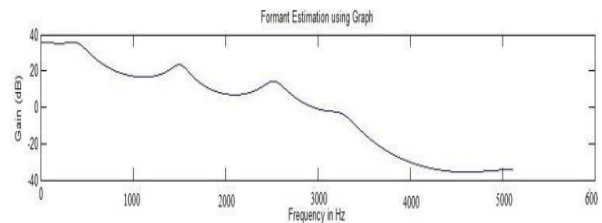
Fig.6. LPC based Formant Estimation
