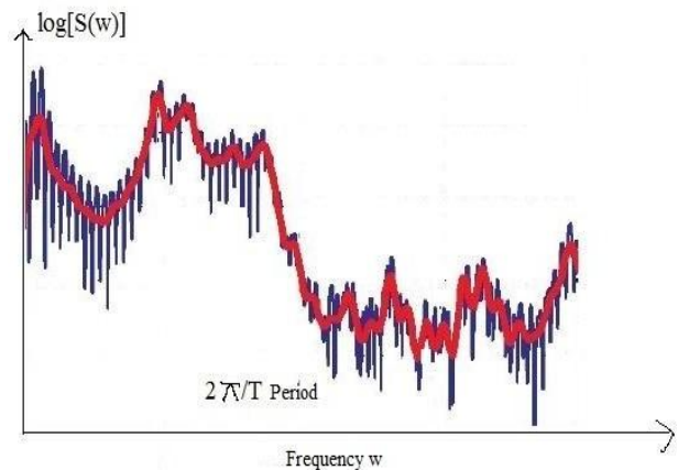
Fig. 1. Pitch component added to the vocal tract Response The periodic component in the logarithmic spectrum at a frequency interval equivalent to the reciprocal of the pitch period T is given by the figure 1. These periodic components are becoming sharp peaks in the cepstrum. In the cepstral domain, the pitch can be estimated by picking the very first peak frequency of the resulting signal within a certain range. The magnitude of the pitch frequency exhibits the emotional level of the speaker.
