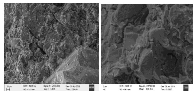
(a)7 days (b)28 days Fig 19. SEM images GGBS based SCBA-2 GPC
