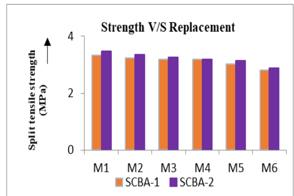
Fig 16. Split tensile strength SCBA-1 and SCBA-2
