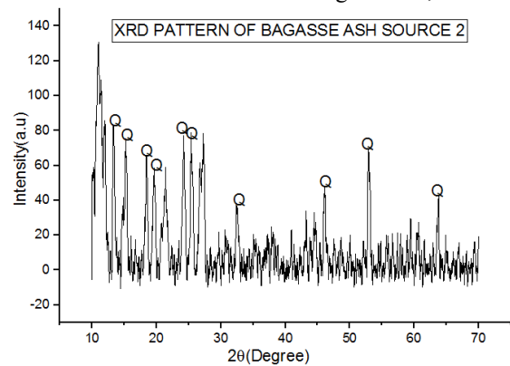
Fig 9. XRD pattern of SCBA-2
