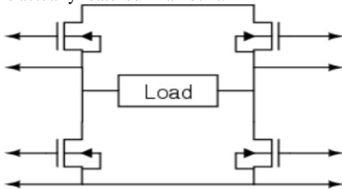
Fig 2. Configuration of H-Bridge
