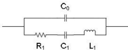
Electrical equivalent circuit
