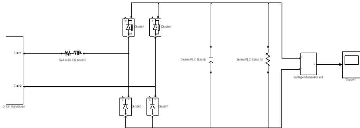
Figure 4.3 Synchronized switch harvesting over inductor
