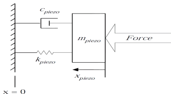
Figure 2.5 Mass Spring Model of Piezoelectric Generator
