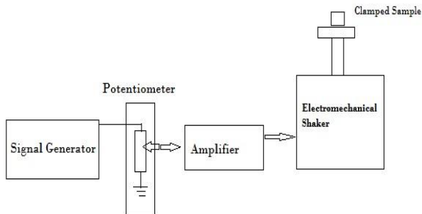
Figure 2.3 Experimental setup of the micro generator
