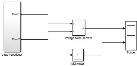
Figure 4.1 Piezoelectric transducer
