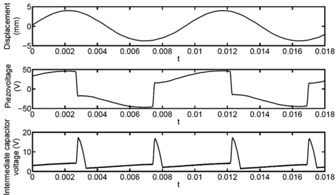
Figure 4.9 Output piezo voltage and Displacement
