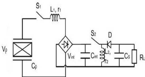
Figure 3.1 Double synchronized switch harvesting model
