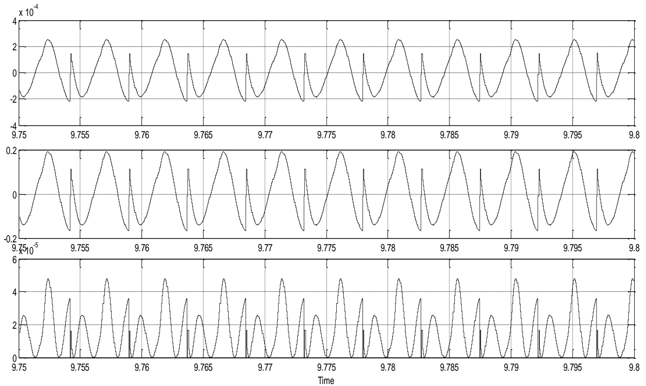
Figure 4.8 Output current, voltage and power without dead zone
