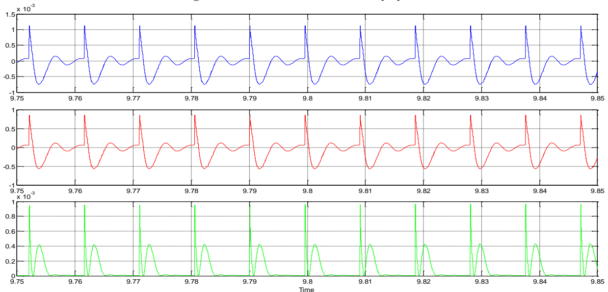
Figure 4.7 Output current, voltage and power with dead zone
