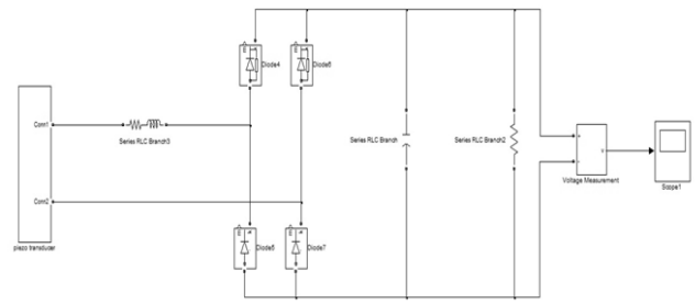
Figure 4.2 Simulation circuit of standard extraction circuit
