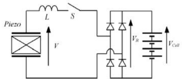
Figure 2.6 Synchronized switch harvesting over inducton
