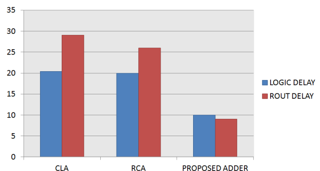
Fig. 6: COMPARISON GRAPH OF LOGIC DELAY AND ROUTE DELAY
