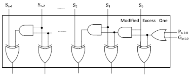
Fig. 2. STRUCTURE OF RIPPLE CARRY ADDER
