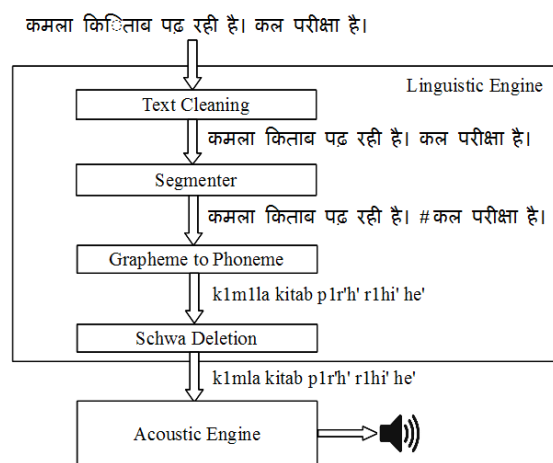
Fig. 1. Text-to-Speech Block Diagram
