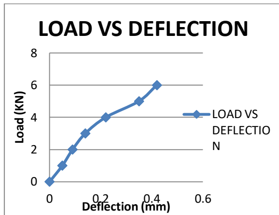
Fig 7: Graph showing load v/s deflection curve
