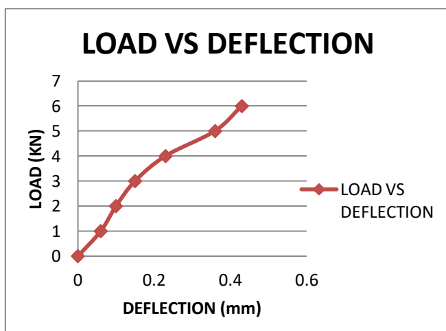
Fig 8: Graph Showing Load Vs Deflection
