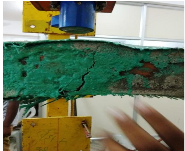
Fig 11: crack pattern on GFRP arches
