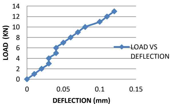
FIG 11 LOAD VS DEFLECTION CURVE
