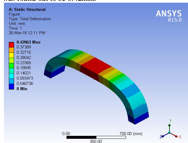
Fig 10: Analytical analysis of arch without GFRP
