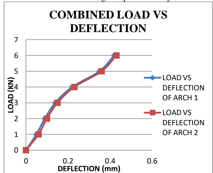
Fig 9: Combined graph showing Load Vs Deflection
