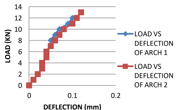
FIG 13 LOAD VS DEFLECTION CURVE
