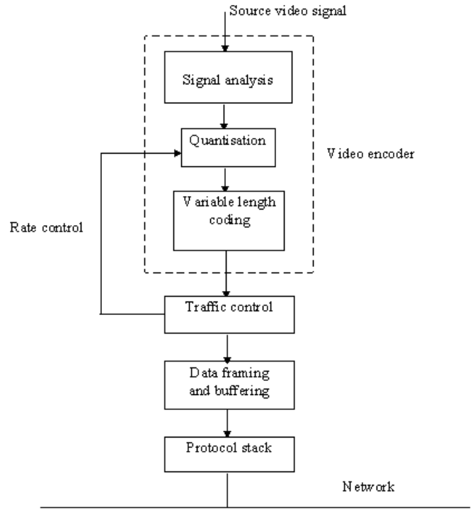
Fig. 2 Functional diagram for video data transmission
