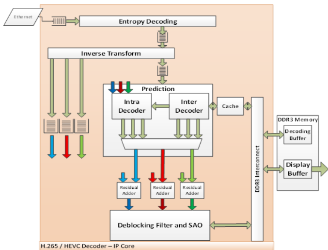
H.265 / HEVC Decoder – IP Core
