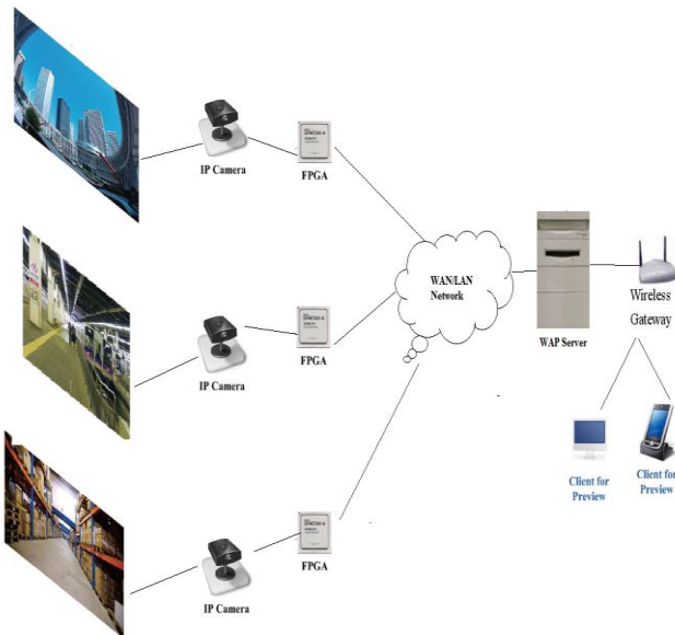
Fig. 1: System Architecture
