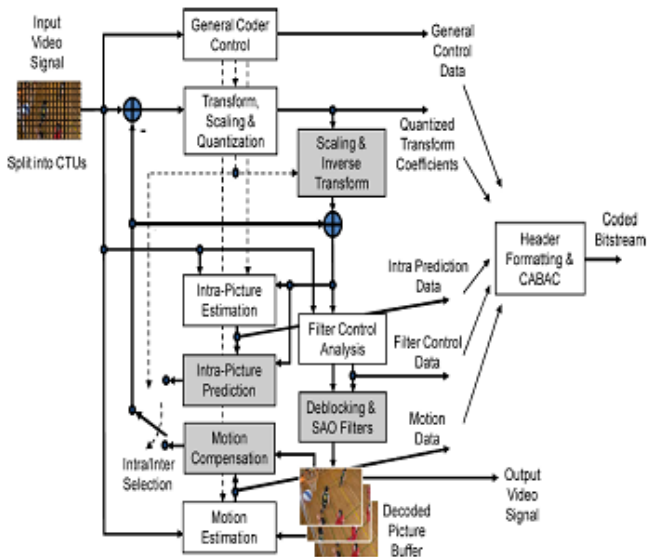
Figure 6: HEVC Encoder
