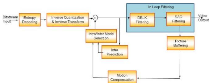
H.265 / HEVC Decoder – IP Core
