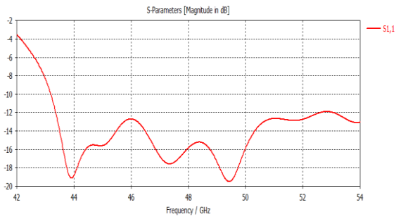
Figure 5: The resonant frequency of UWB based SIW antenna
