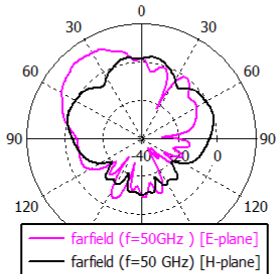
Figure 7: the radiation patterns of selected frequencies
