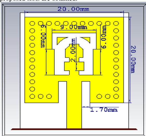
Figure 3: the SIW antenna structure
