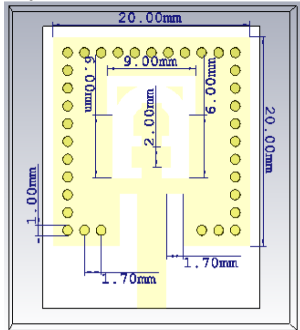
Figure 4: The substrate structure
