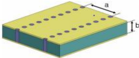
Figure1: Structure of SIW [2].
