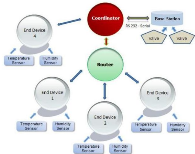
Figure 3: The basic topology of monitoring system
