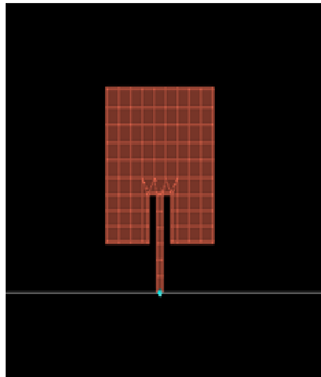
Fig. 5. Design of unshorted microstrip patch antenna
