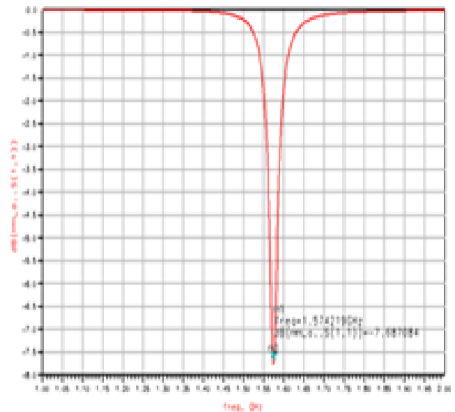
Fig. 6. Simulation result for unshorted microstrip patch antenna
