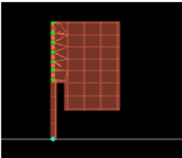
Fig. 9. Design of shorted microstrip patch antenna
