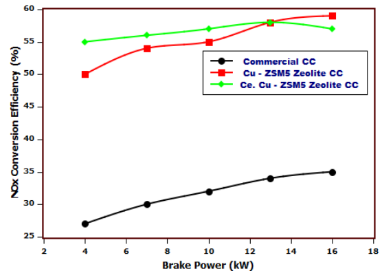
Fig.6 Percentage reduction of NOx Vs load
