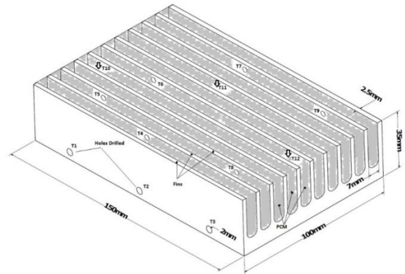
Figure 2: Heat Sink with PCM
