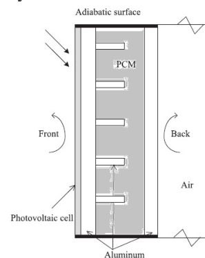
Figure 1 . Schematic of PV-PCM system
