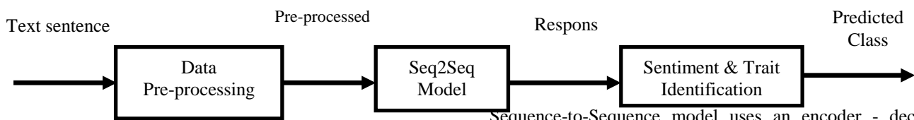
Fig 1.1 System Architecture
