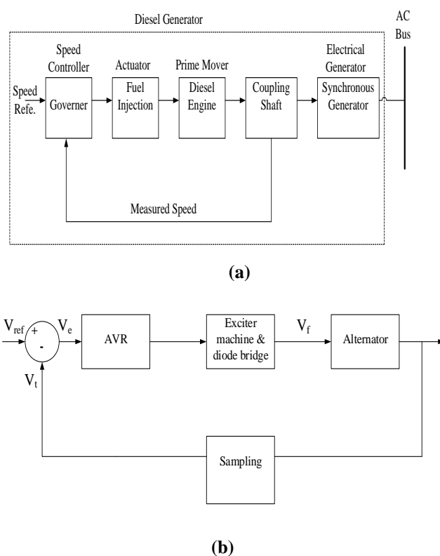
Fig. 1 Control scheme of diesel generator (a) Governor control scheme (b) Excitation Control scheme
