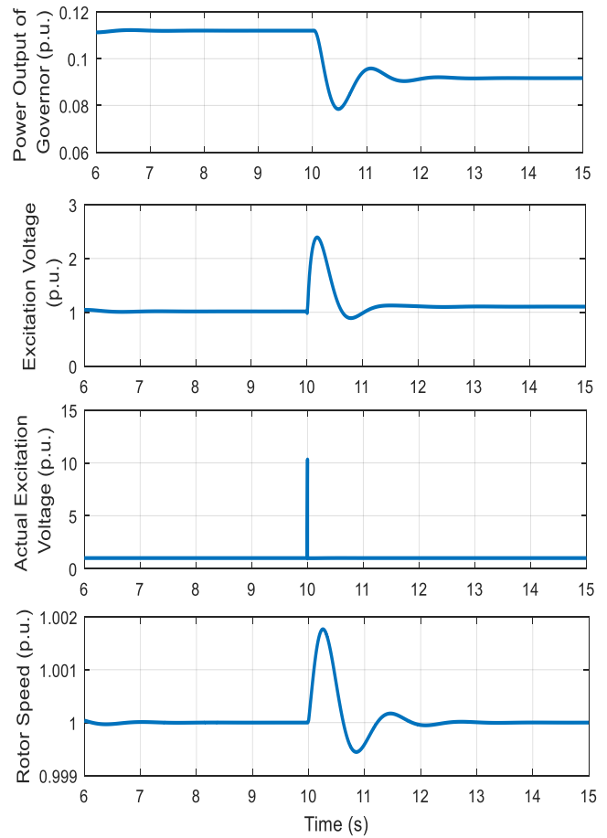
Fig. 10 Waveforms of the turbine output power, exciter output voltage, actual exciter voltage and rotor speed (p.u. values)
