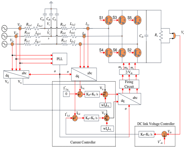
Fig. 16 Closed loop control scheme of UPFR
