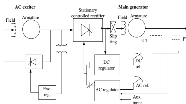
Fig. 4 Voltage source controlled static rectifier excitation system
