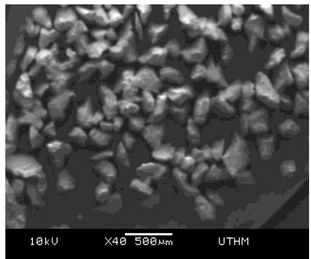
Figure 7 SEM image for fine sand
