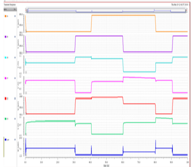
Fig.8 Transient and power analysis
