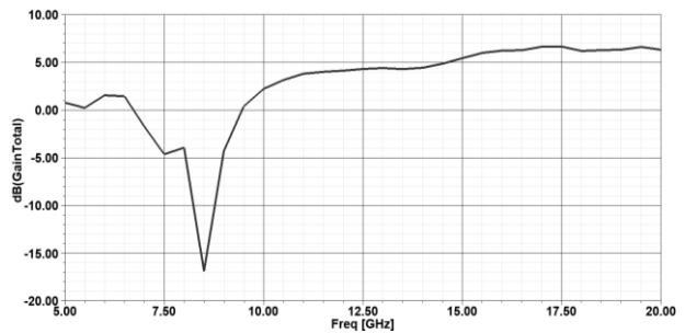
Fig. 10. Frequency vs. Gain.
