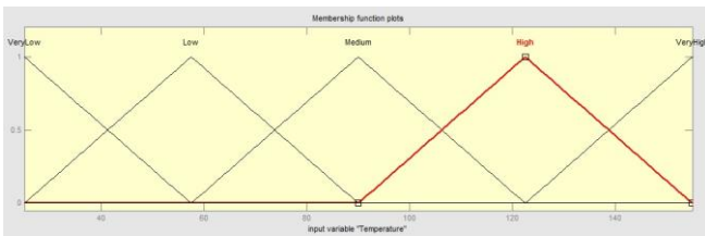
Figure 9 Membership function for input variable ‘temperature’
