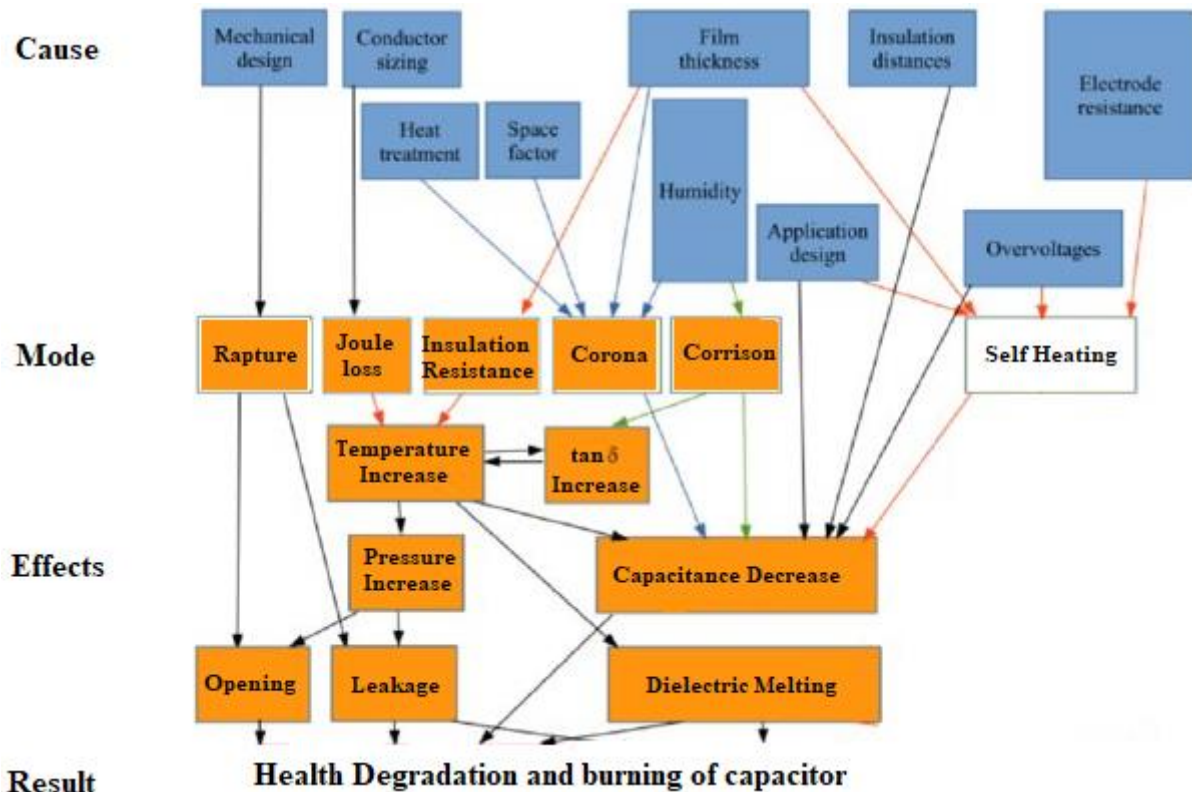
Figure.3 Cause and effect diagram for ceramic capacitor failure
