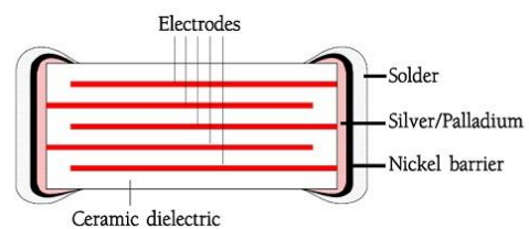
Figure.1 Structure of a ceramic capacitor
