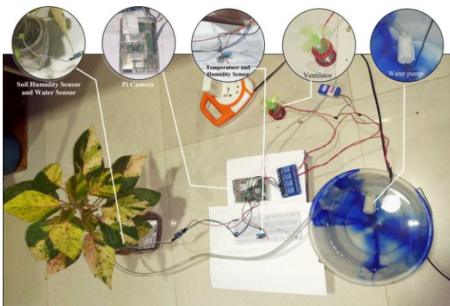
Fig. 8: Prototype arrangement
