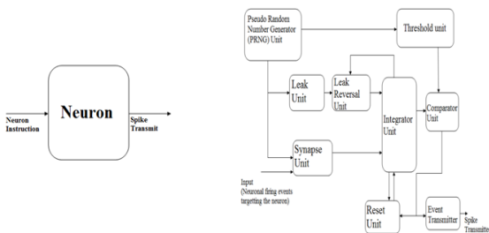
Fig. 7: Neuron Block Diagram
