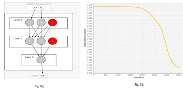
Fig. 8: (a) Network Structure for 2 input XOR, (b) Training Graph
