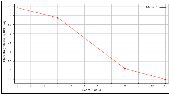
Figure 10. S-Ncurve for Carbon steel
