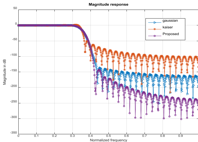
Figure 12: spectral analysis of FIR low pass filter design by using Gaussian, Kaiser and proposed window
