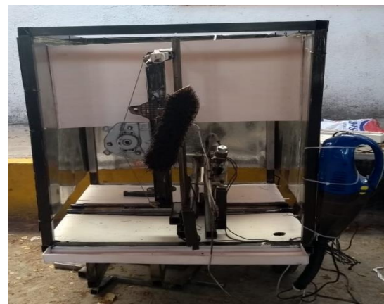
Fig.3. (Front View)
