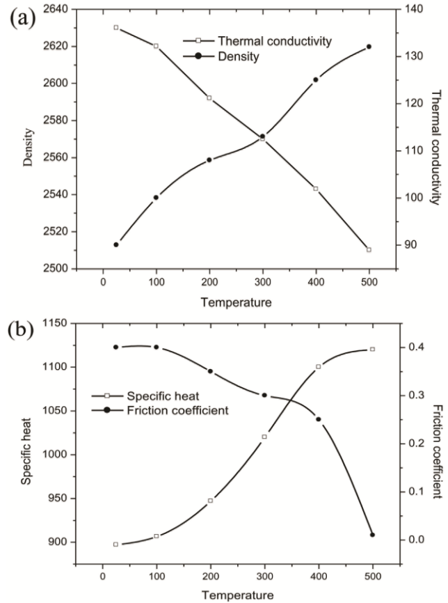
Fig. 4 Temperature dependent material properties of third generation Al-Li alloy [19]
