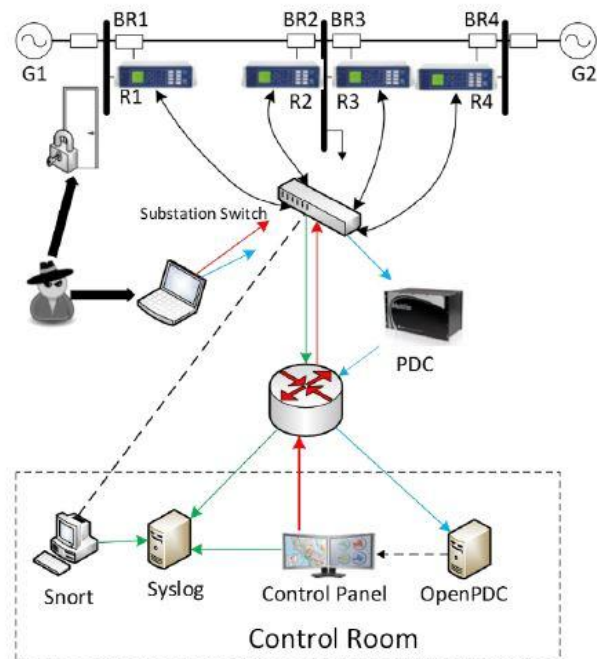
In Figure-1 Power System Framework
