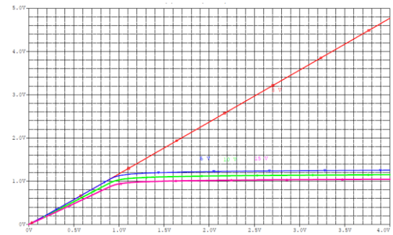
Fig. 4 V_{ce} vs V_s characteristic at constant V_g
