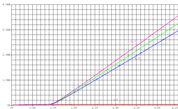
Fig. 3 I_c vs V_s characteristic at constant V_g
