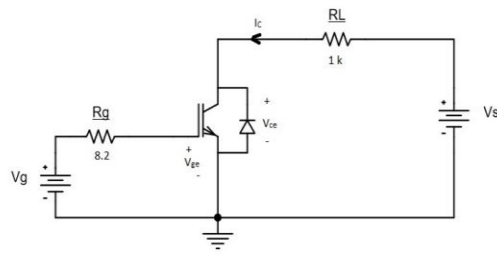
Fig. 2 Test circuit of BiMOSFET
