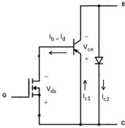
Fig. 1 Equivalent Circuit of BiMOSFET
