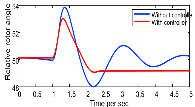
Fig. 12 Relative rotor angle deviation of generators during increase in load
