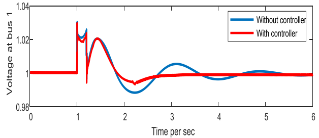
Fig. 19 Voltage Stability during decrease in load
