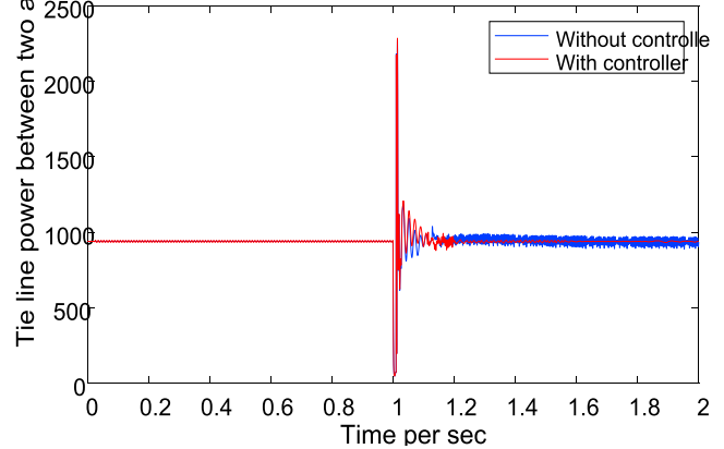
Fig. 6 Tie Line Power between two areas
