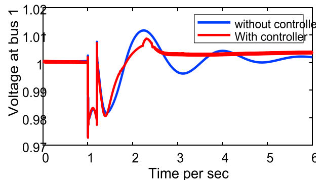
Fig. 13 Voltage Stability during increase in load
