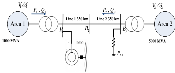
Fig. 1 Two machine two-area test system
