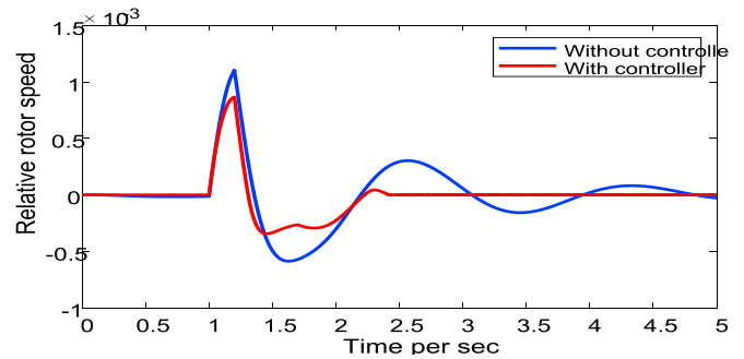
Fig. 10 Relative rotor angle deviation of generators during an increase in load
