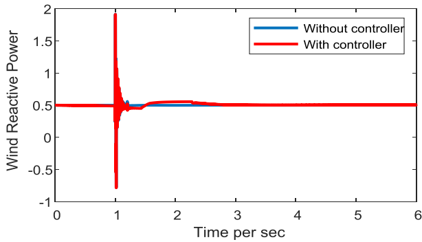
Fig. 21 Dynamic response of wind reactive power during decrease in load
