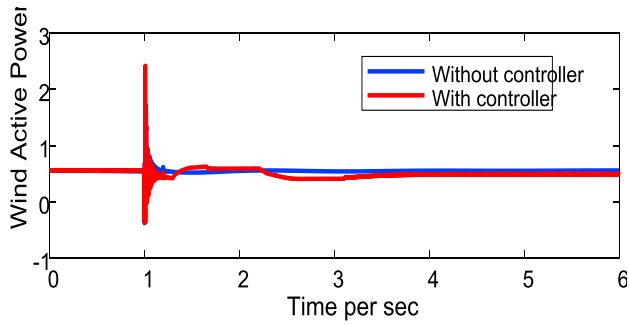
Fig. 14 Dynamic response of wind active power during increase in load
