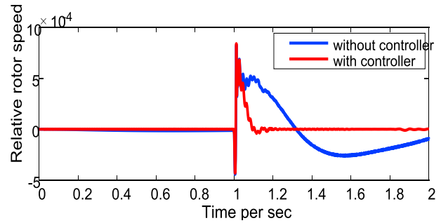
Fig. 5 Relative rotor speed deviation of generators
