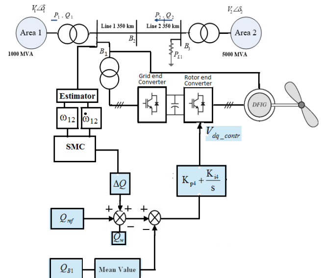
Fig.3 Two Area Power System with SMC
