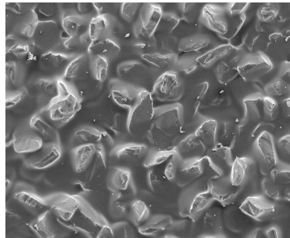
Fig 3: Surface Morphology of emery paper before wear test
