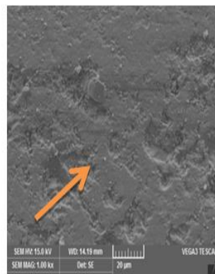
Fig 4h : 0.4wt% Al-G
