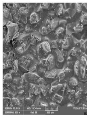
Fig 5b: 0.2wt% Al-G
