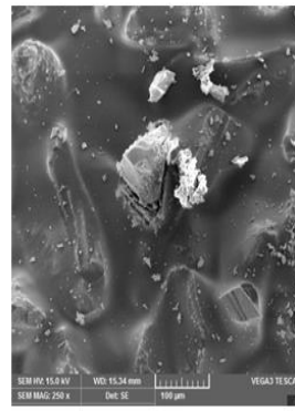
Fig 5c: 0.3wt% Al-G
