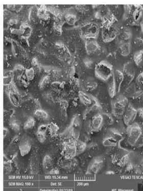
Fig 5a: 0.1wt% Al-G
