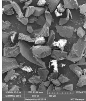
Fig 7b: 0.2wt% Al-G samples
