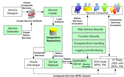
Figure 2: Oracle E-Business Suite Integrated SOA Gateway Architecture[29]
