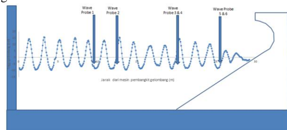
Figure 6. Schematic of hydraulic experimental model
