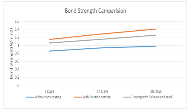
Fig. V Day Wise Bond Strength Comparison
