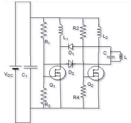
Fig. 3. Oscillator Circuit for WPT
