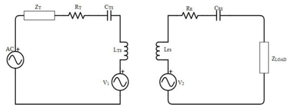
Fig. 2. Equivalent circuit of inductive coupling with voltage drop due to mutual impedance
