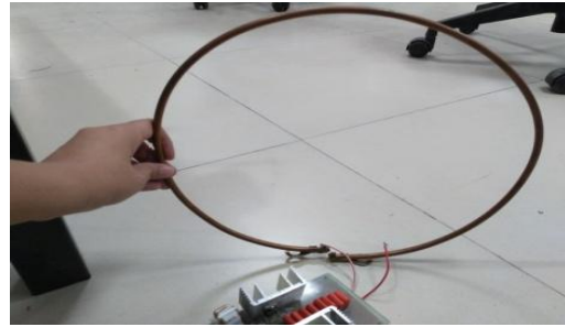
Fig. 5. Receiving Coil
