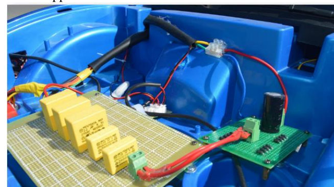
Fig 6: Secondary Capacitor bank & High Frequency Rectifier
