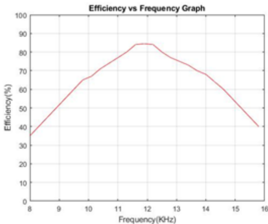
Fig 9: Efficiency vs Frequency graph
