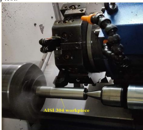
Figure 2 Experimental set for machining test
