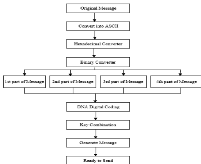
Fig.4 Encryption Process
