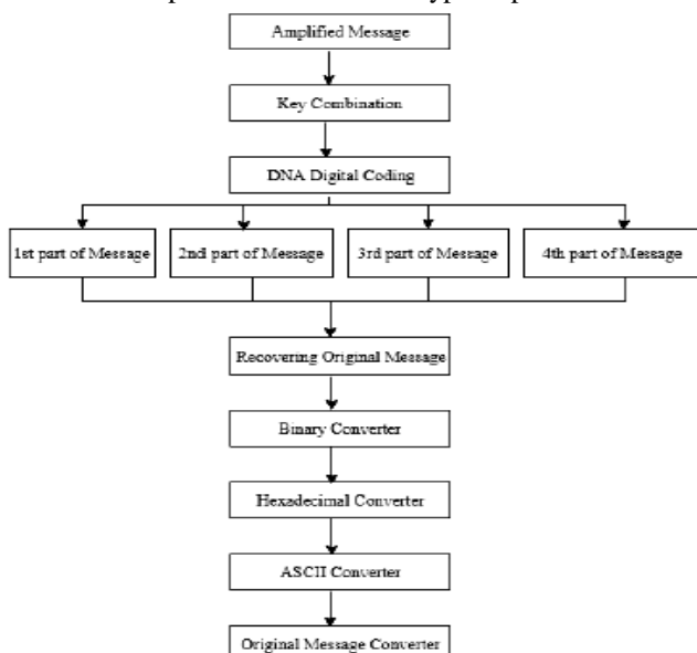
Fig.5 Decryption Process
