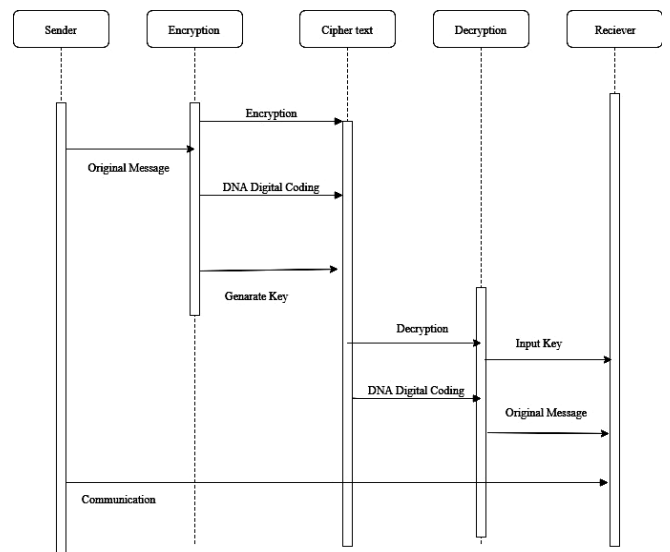
Fig.3 Sequence Diagram
