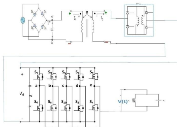
Fig.2 Schematic Diagram Synthesized Multilayer Power Converter
