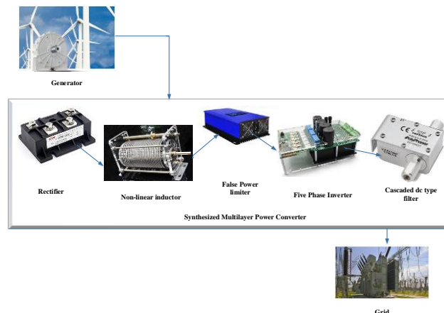
Fig. 1 The flow diagram of new model
