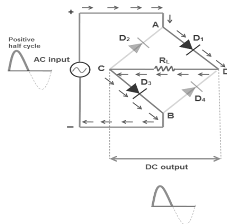
Fig. 4 The positive half cycle of rectifier
