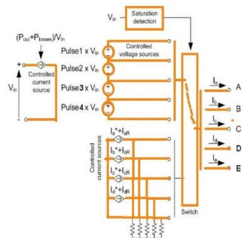
Fig. 8 Five phase inverter
