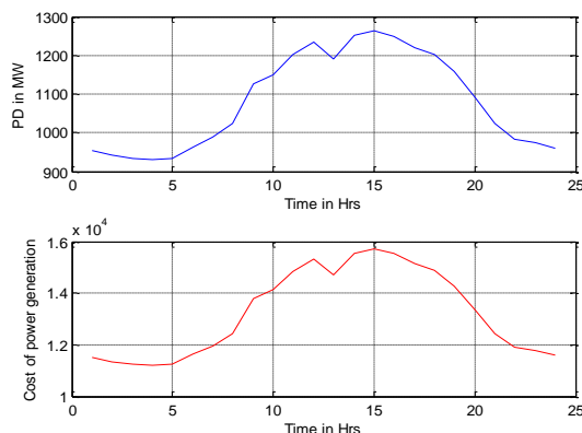
Fig 2: Time (Hrs) Vs Fuel cost (Rs/Hr) and load
