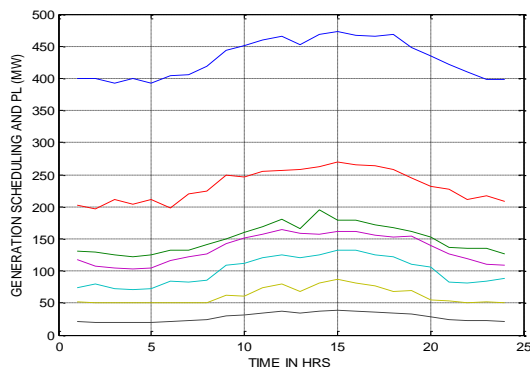
Fig 1: Time in Hrs Vs Generation scheduling and losses in MW
