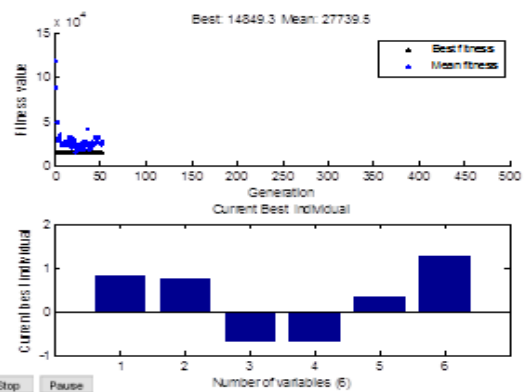
Fig 3: Generation Vs Fitness value (Best & Mean)
