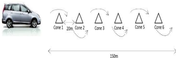
Fig. 2 - Schematic of the test track
