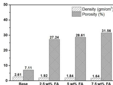
Fig. 7 Comparison of Porosity values between base and composites.
