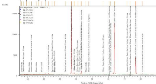
Fig. 3 XRD spectrum of AA7075-Si 3 N 4 -FA composite.
