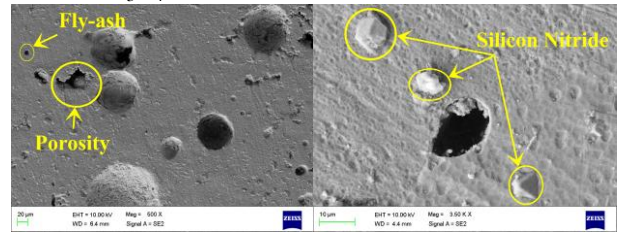
Fig. 4 (a) & (b) SEM Images of AA7075-Si 3 N 4 -FA composite.
