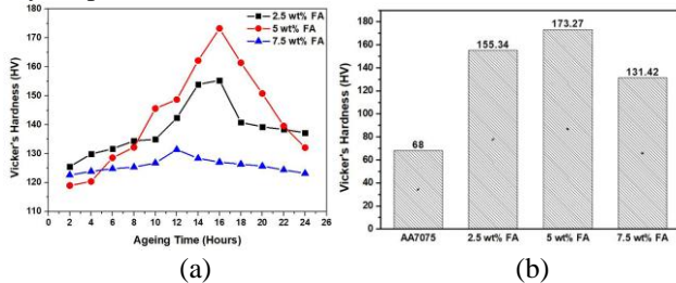
Fig. 6 (a) Microhardness for 24 hours Ageing period. (b) Hardness comparison between base and composite.
