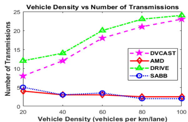
Fig. 7 Number of Transmission
