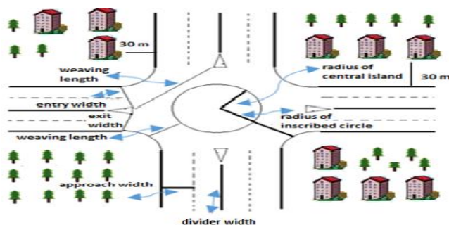
Fig. 3 Rotary intersection/junction with design elements
