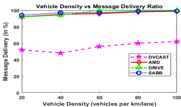
Fig. 5 Message Delivery Ratio
