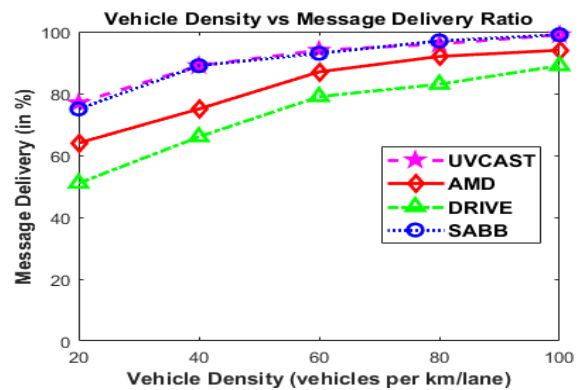
Fig. 9 Message Delivery Ratio
