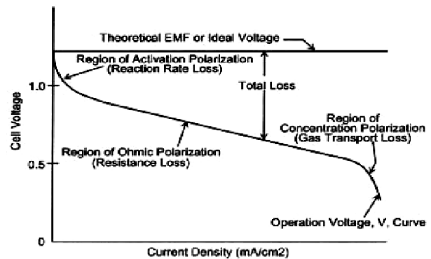
Fig1 Cell Voltage Vs Current Density
