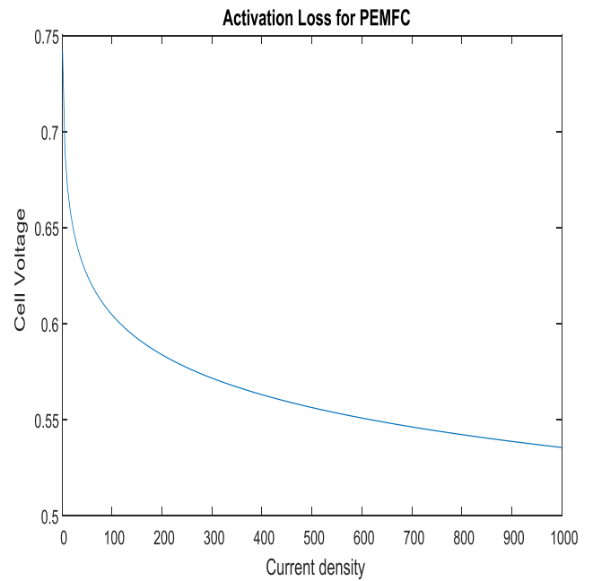
Fig 3.2. Activation Loss graph
