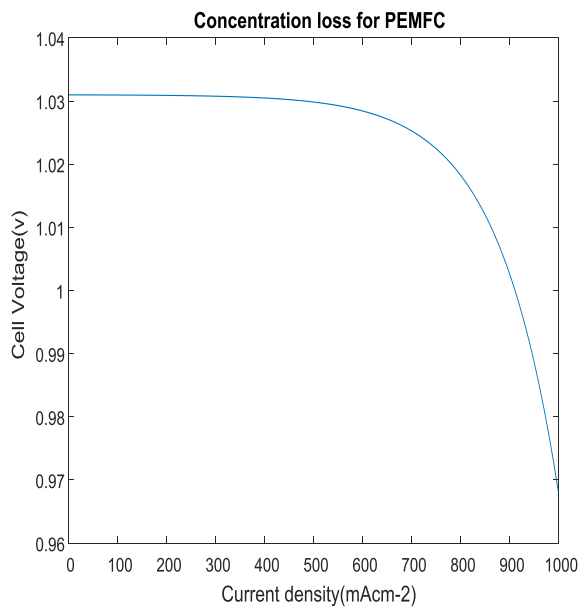
Fig 3.4 Concentration Loss graph
