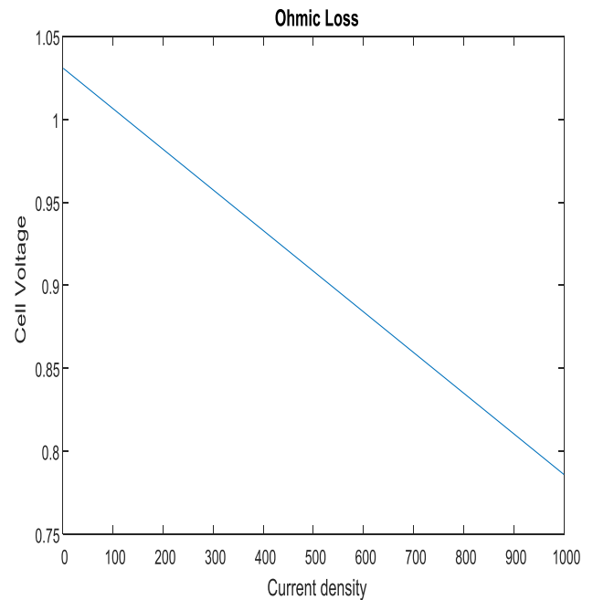
Fig 3.3 Ohmic Loss graph
