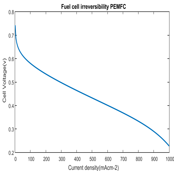
Fig 3.1. Cell Voltage vs Current density
