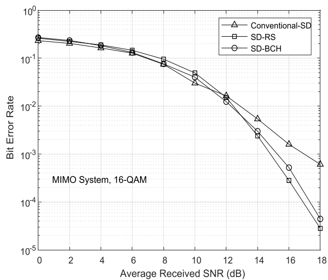
Fig. 4. The BER vs. SNR with a 4 \times 4 MIMO system for 16-QAM mapping
