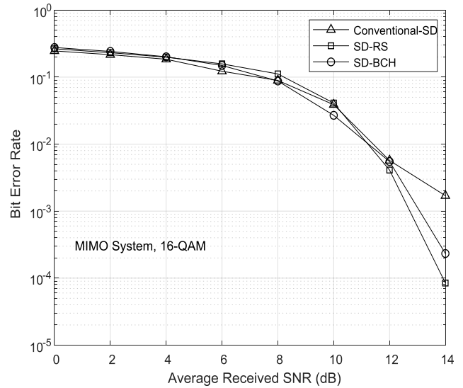
Fig. 5. The BER vs. SNR with a 8 \times 8 MIMO system for 16-QAM mapping
