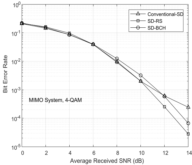
Fig. 2. BER vs. SNR with a 4 \times 4 MIMO system for 4-QAM mapping
