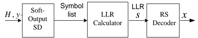
Fig.1. MIMO detection at receiver
