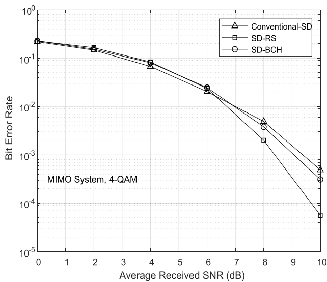
Fig. 3. The BER vs. SNR with a 8 \times 8 MIMO system for 4-QAM mapping
