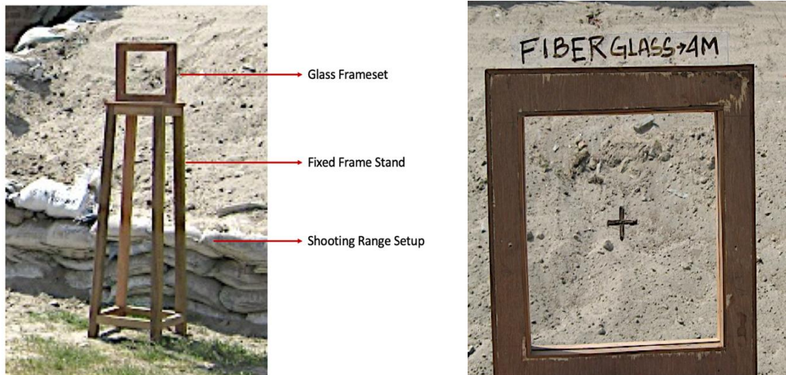
Figure 1-2- Demonstration of the setup for the shooting with a changeable glass frameset.
