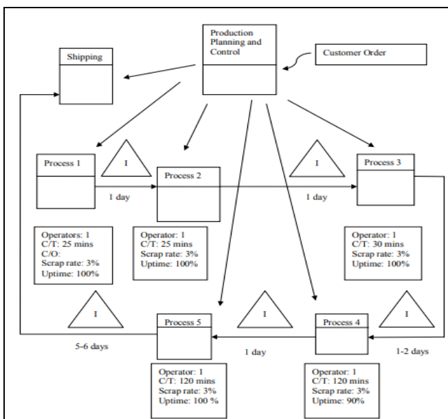
Fig. 1: Current State Map of OSM300 Assembly Process
