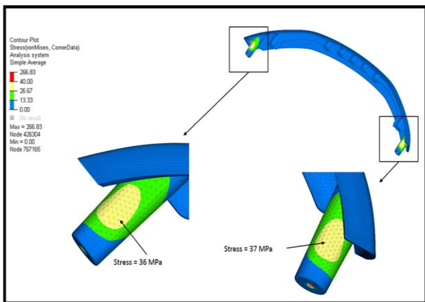
Figure 2. Stress distribution for the entire setup
