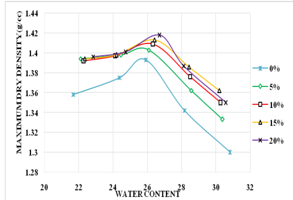
Figure 1. Compaction Characteristics Curve for Treated Soil Sample with Addition of Different Proportions of Dunite Powder
