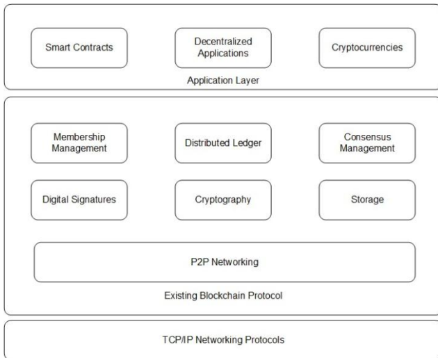
Fig. 1. Generalized sectional view of Blockchain protocol stack
