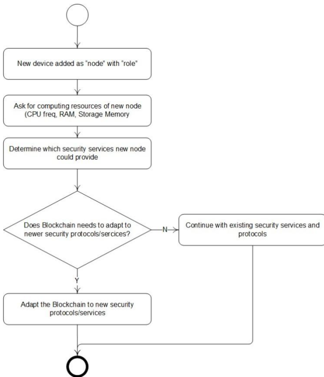
Fig. 2. Snapshot of the adaptive module in main node when a new device is added to the Blockchain
