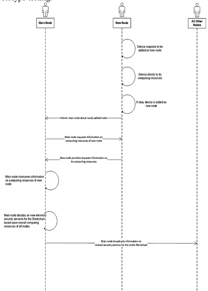
Fig. 3. Interactions between main device and all the other nodes
