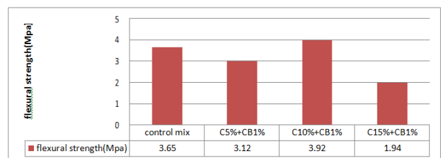
Fig 6: Flexural Strength Results With Other Cementitious Material And Different Percentages
